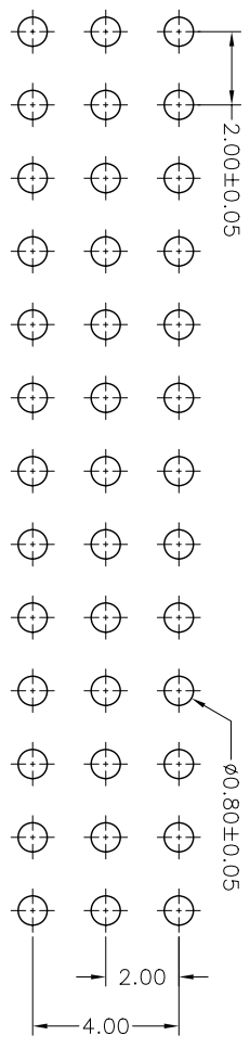
Recommended PCB Board Hole Layout
