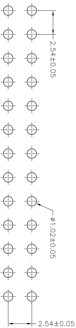
Recommended PCB Board Hole Layout
